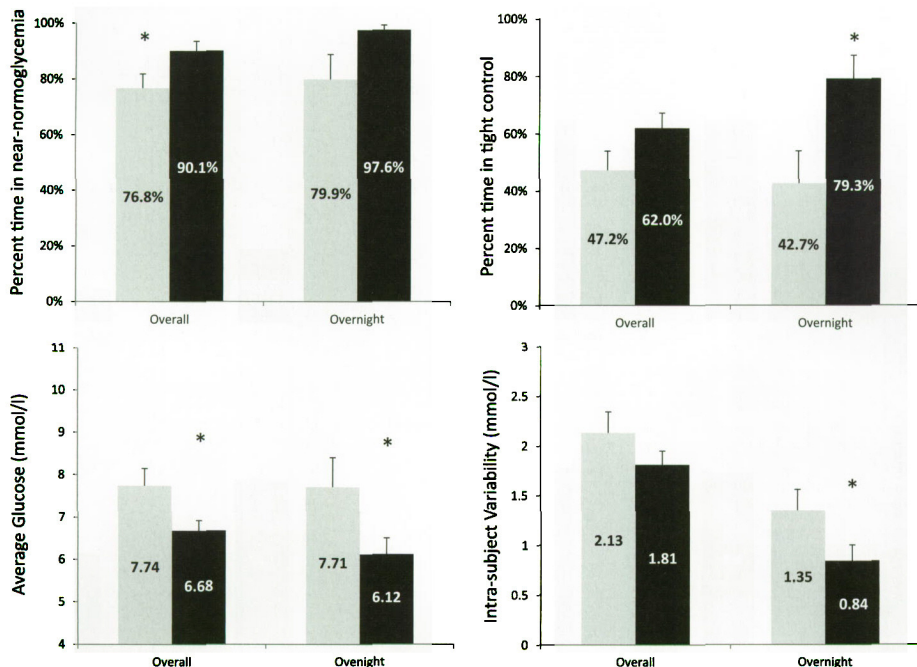
FIG. 4. Primary outcomes of eCTR: Time in near normoglycemia (3.9–10 mmol/L) and tight control (4.4–7.78 mmol/L), average glucose, and intra-subject variability during open- and closed-loop admissions, contrasted by overall and overnight periods. * P < 0.05 . Open-loop CSII, gray bar; eCTR, black bar.
